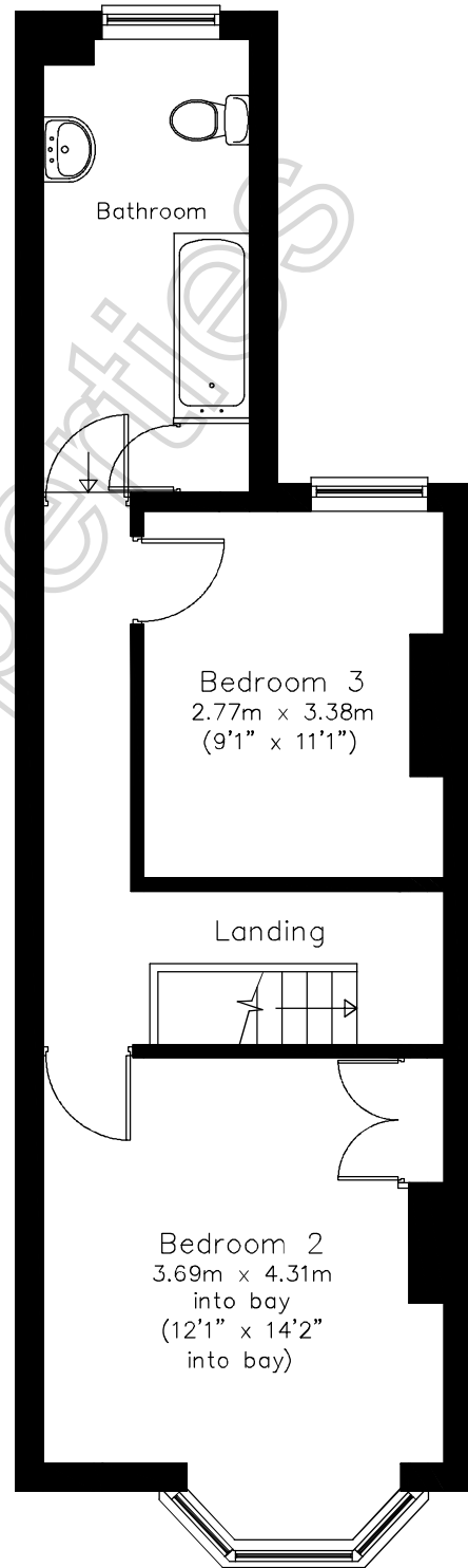
FIRST FLOOR
